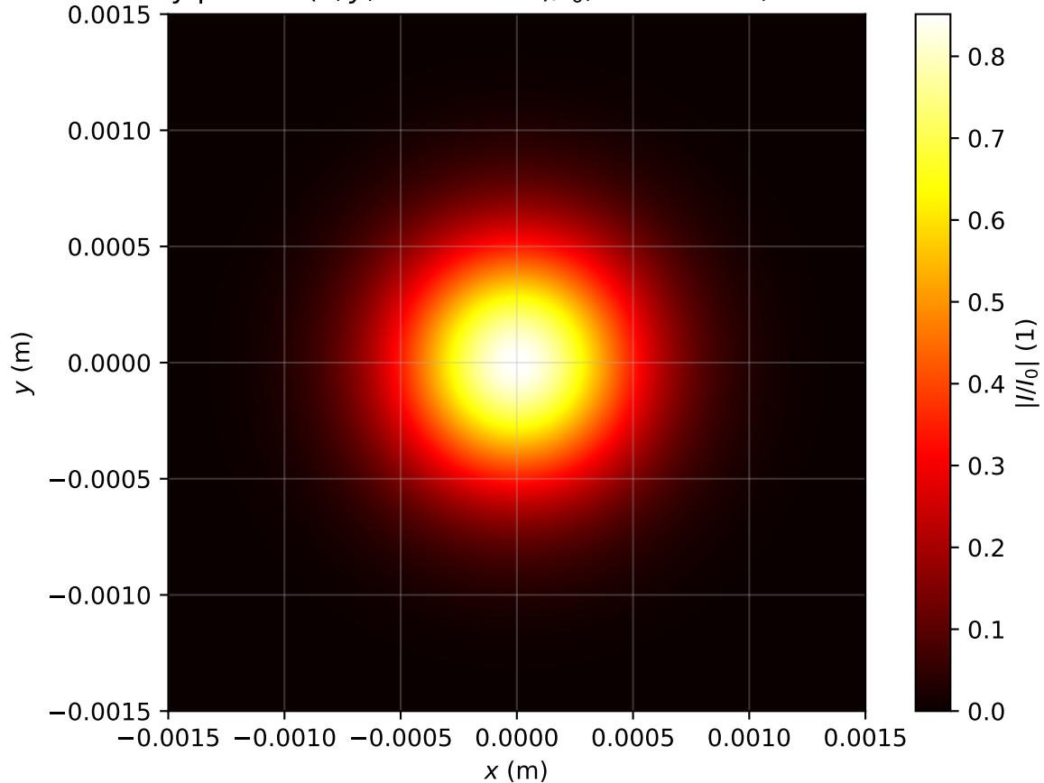
Intensity profile I(x, y, z = 1.115m)/I_0 , Pin=0.2Pcr, artificial time
